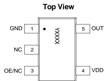
Figure 1. Pin Assignments
